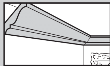
CROWNS: USED WHERE WALLS & CEILING MEET. USED TO COVER LARGE ANGLES. ALWAYS SPRUNG.
